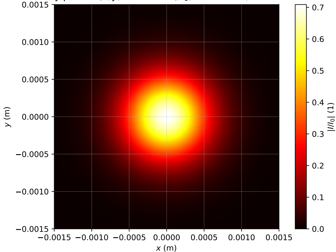
Intensity profile I(x, y, z = 2.070m)/I_0 , \text{Pin}=0.4\text{Pcr} , artificial time
